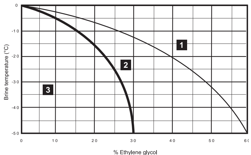
Figure 4 - Freezing point versus ethylene glycol percentage
