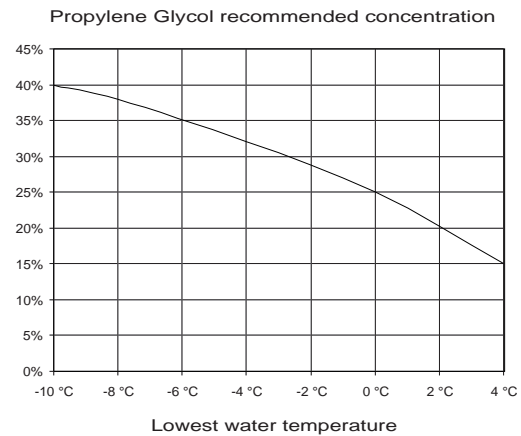
Figure 7 - Propylene glycol recommended concentration
