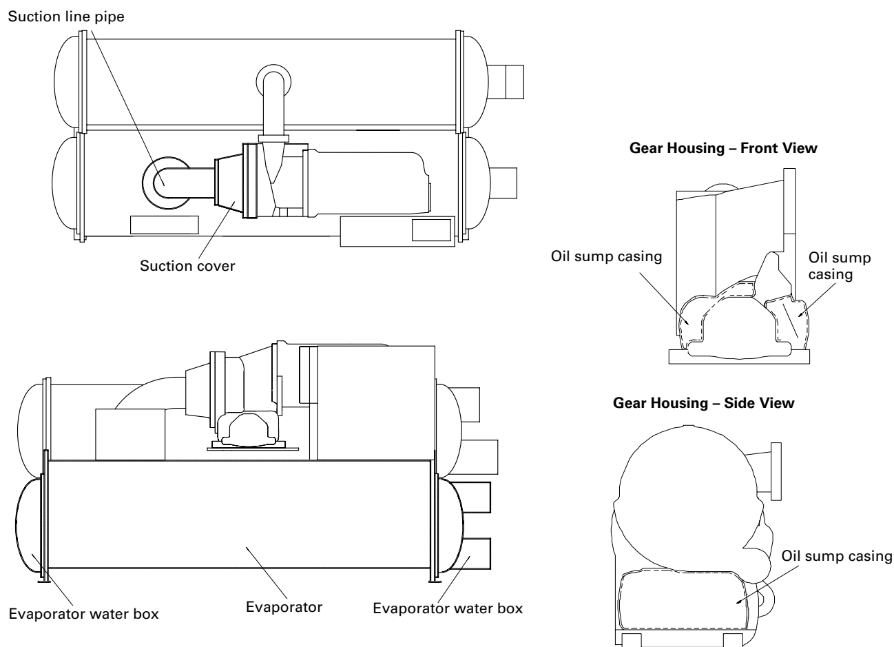
Figure 25. Typical CVGF insulation requirements Insulate where dotted lines are indicated.
