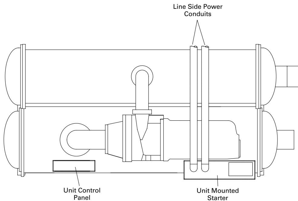
Figure 28. Typical equipment room layout with unit-mounted, Wye-Delta
