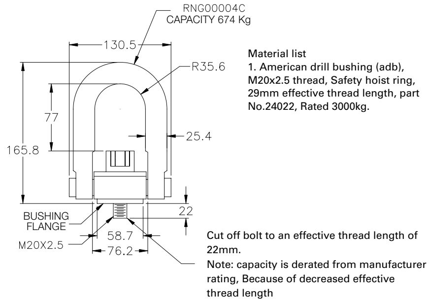
Figure 23 : Eyebolt connection (Safety hoist ring M20X2.5)
