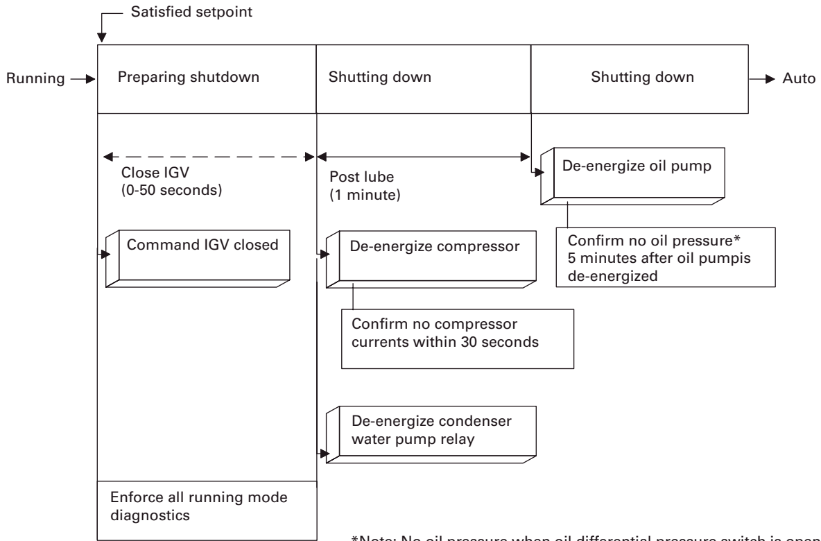
Figure 11. CVGF sequence of operation: satisfaction setpoint
