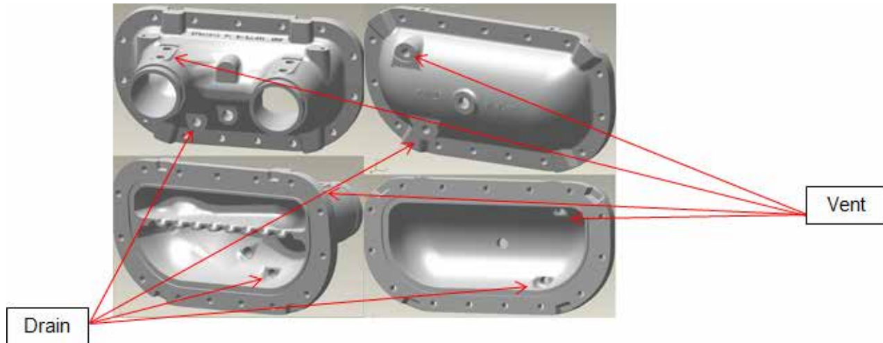
Figure 4 – Drain and vent position on evaporator
