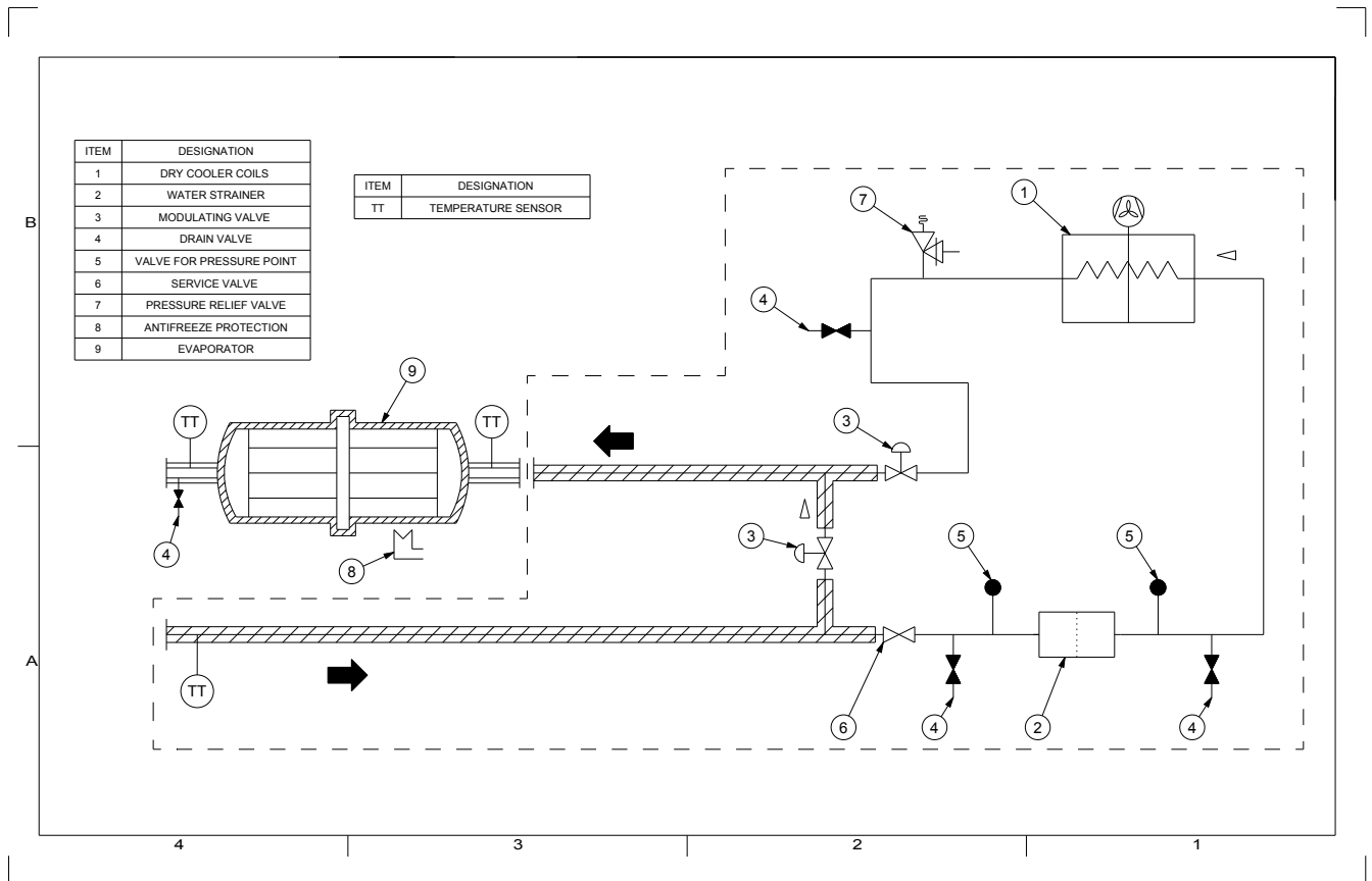
Figure 21 – Flow chart – Free-Cooling – Direct free cooling version
