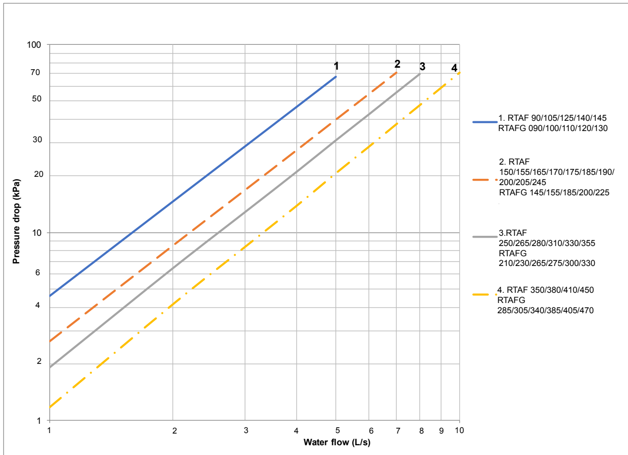
Figure 18 – Water pressure drop - heat recovery heat exchanger
