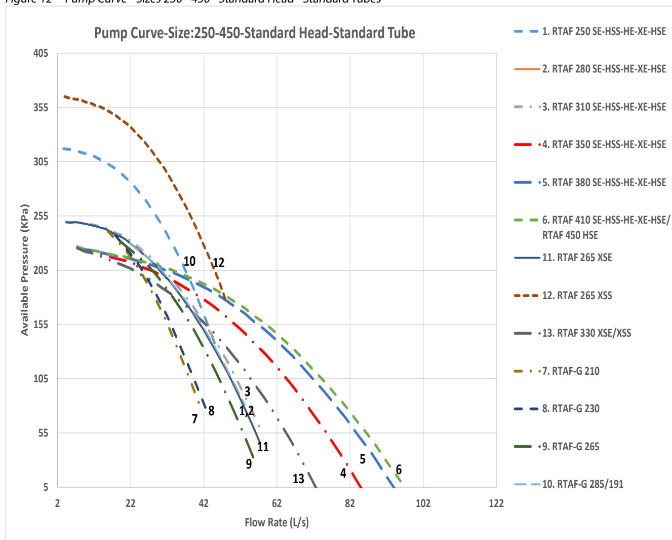
Figure 12 – Pump Curve - Sizes 250 - 450 - Standard Head - Standard Tubes
