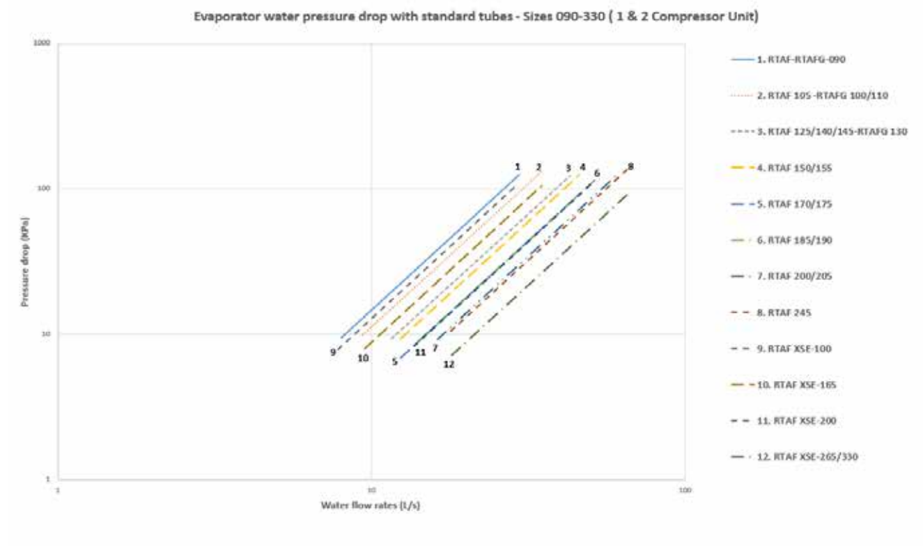
Figure 6a – Evaporator water pressure drop with standard tubes - Sizes 090-330
