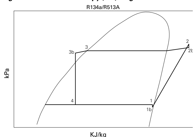
Figure 34 – Pressure enthalpy (P-h) diagram
