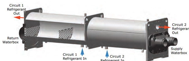
Figure 2 - CHIL Evaporator
