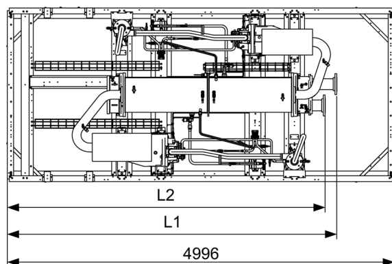
Top View(With fan /coil removed)
