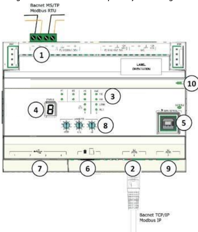
Figure 1 - Wiring locations and connection ports of Thermologic controller
